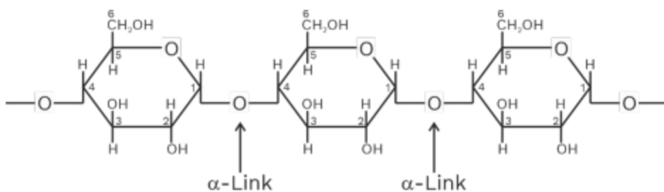
Amylose
