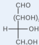
D-Aldopentose
