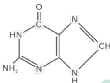
Guanine (G)
