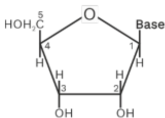
Nucleoside
