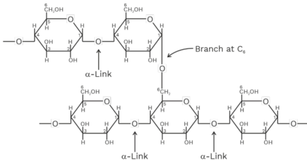
Amylopectin
