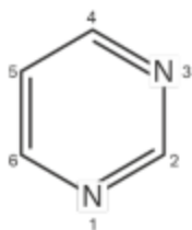
Pyrimidine
