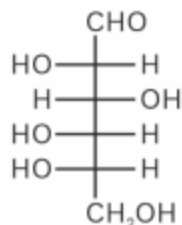
L-Glucose
