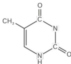
Thymine (T)
