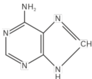
Adenine (A)
