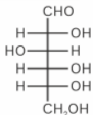
D-Glucose
