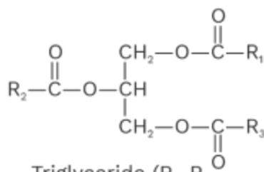
Triglyceride ( \text{R}_1 , \text{R}_2 and \text{R}_3 are fatty acids)
