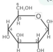
\beta -D(+)-Glucose
