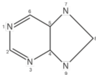
Purine
