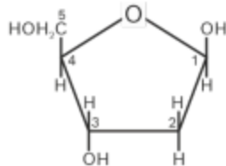
\beta -D-2-deoxyribose
